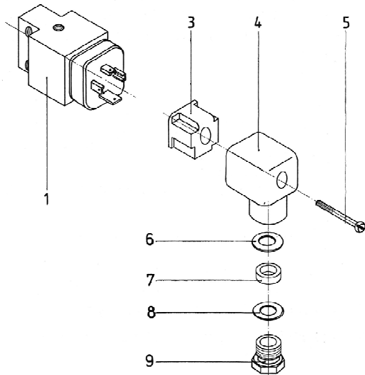
Fig. 11 Explosion drawing contact K 18
