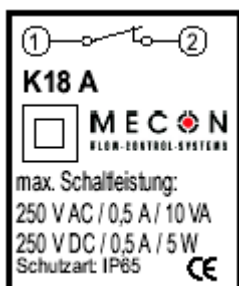
Fig. 7 Contact K 18 A
