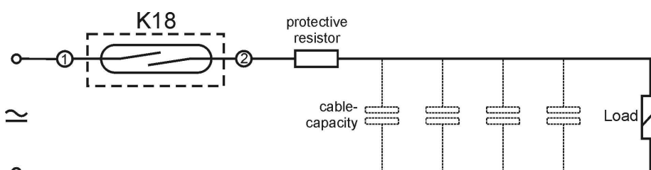
Fig. 9 Protective circuit for current limitation
