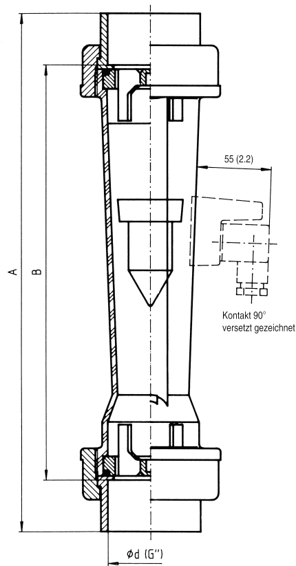
Fig. 5 Troglux, Dimensions in mm
